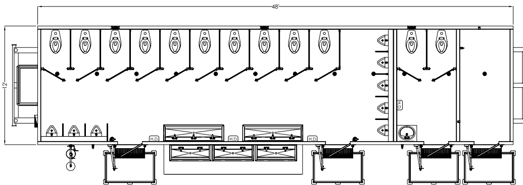
The Reliever Rig Floor Plan
